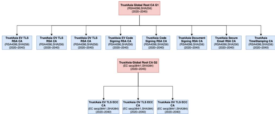
TrustAsia certificate architecture
